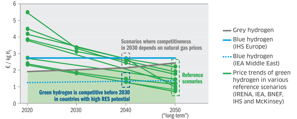
HYDROGEN PRODUCTION COSTS IN THE MAIN BENCHMARKS
