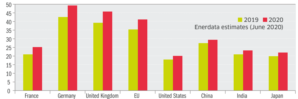
SHARE OF RENEWABLE SOURCES* IN ELECTRICITY GENERATION BY COUNTRY
