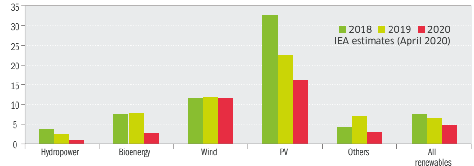
ANNUAL GROWTH IN GLOBAL RENEWABLE ELECTRICITY GENERATION BY SOURCE
