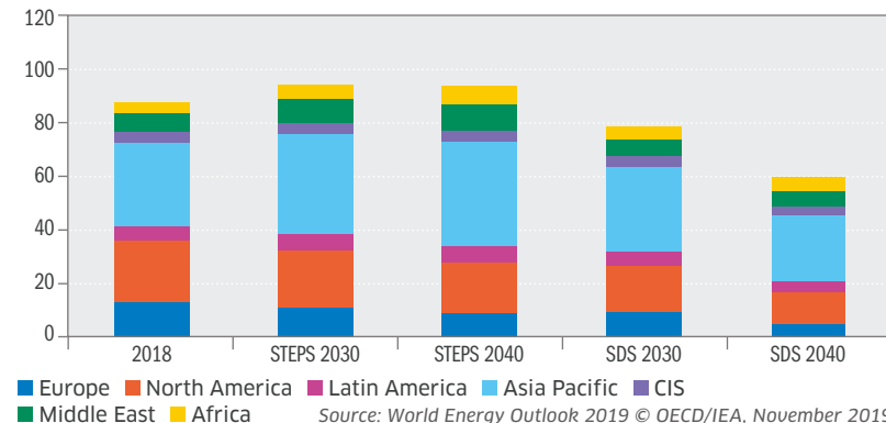
FORECAST OF OIL PRODUCTION IN THE STATED POLICIES SCENARIO AND SUSTAINABLE DEVELOPMENT SCENARIO, IEA 2019 (MB/D)
